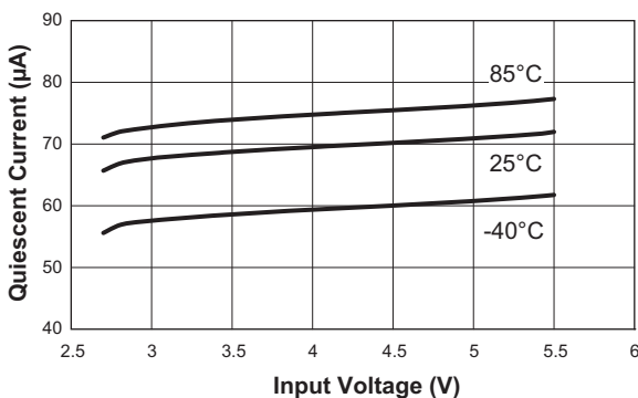
No Load Quiescent Current vs. Input Voltage ( V_{EN1} = V_{EN2} = V_{IN} )
