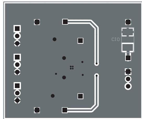
Figure 4: AAT2713 Evaluation Board Bottom Side.
